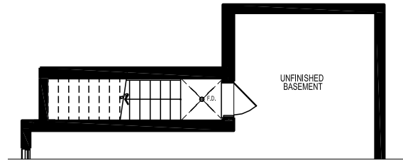
PART. BASEMENT WITH OPT. WALK-UP STAIR Elevation B
